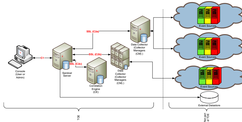
Figure 2 – Sentinel 8.1 Configuration with External Datastore
