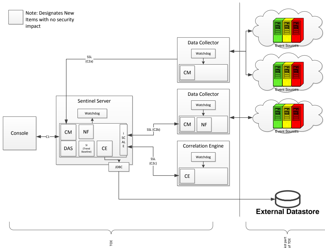
Figure 7 – TOE Boundary
