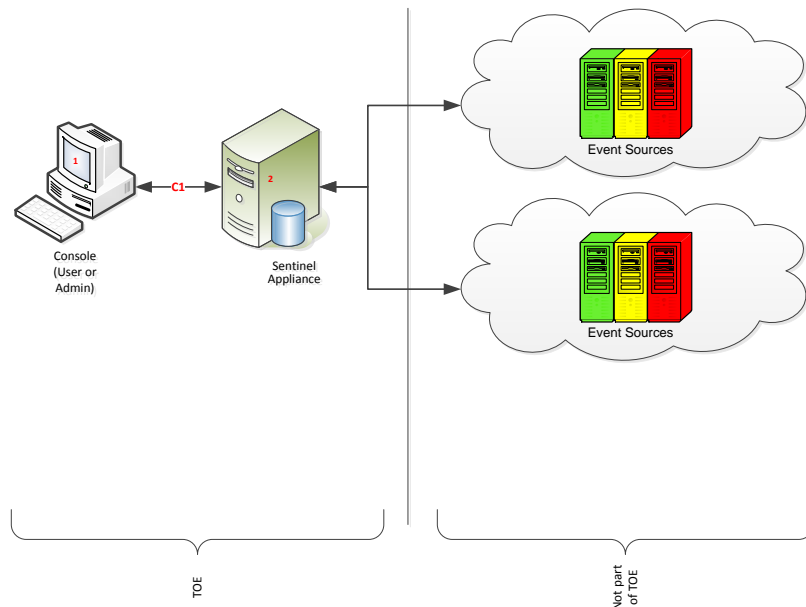
Figure 3 – Sentinel 8.1 Appliance Configuration
