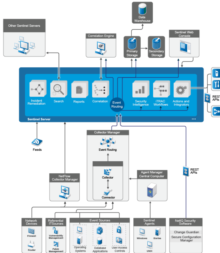
Figure 5 – Sentinel Conceptual Architecture
