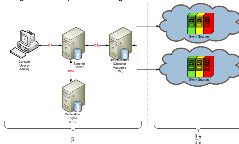
Figure 1 – Basic Sentinel 8.1 Configuration
